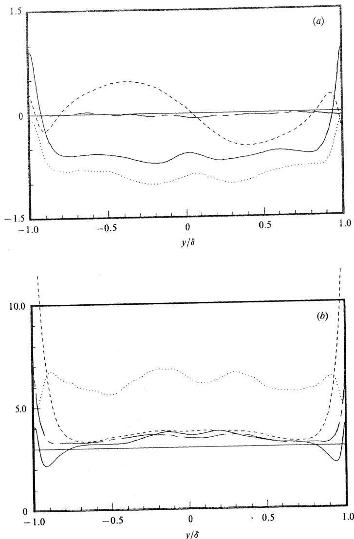
FIGURE 18. Skewness and flatness factors in global coordinates. (a) Skewness, —, S(u') ; ---, S(v') ; — · —, S(w') ; ·····, S(p') . (b) Flatness, —, F(u') ; ---, F(v') ; — · —, F(w') ; ·····, F(p') .
