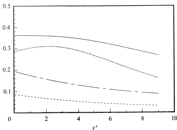
FIGURE 12. Near-wall behaviour of Reynolds stresses: —, u_{\text{rms}}^+/y^+ ; ---, w_{\text{rms}}^+/y^+ ; ----, 10v_{\text{rms}}^+/y^{+2} ; ·····, 400(-u'v')/y^{+3} .
