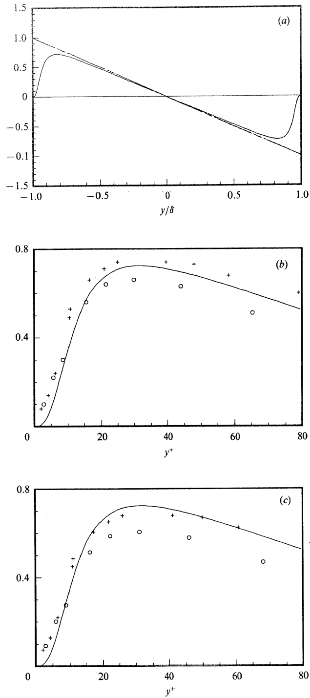
FIGURE 10. Reynolds shear stress normalized by the wall shear velocity: (a) in global coordinates, —, -\overline{u'v'} ; ---, -\overline{u'v'} + (1/Re)\partial\bar{u}/\partial y ; - · - · -, total shear stress for fully developed channel; (b) in wall coordinates, —, -\overline{u'v'} ; ○, data from Eckelmann (1974) for Re_\tau = 142 ; +, data from Eckelmann for Re_\tau = 208 ; (c) same as (b) except the data are renormalized by 'corrected' u_\tau .
