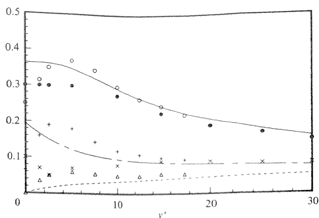
FIGURE 8. Turbulence intensities near the wall normalized by the local mean velocity: —, u_{\text{rms}}/\bar{u} ; ---, v_{\text{rms}}/\bar{u} ; — · —, w_{\text{rms}}/\bar{u} . From Kreplin & Eckelmann (1979): \circ , u_{\text{rms}}/\bar{u} ; \triangle , v_{\text{rms}}/\bar{u} ; +, w_{\text{rms}}/\bar{u} . From Hanratty, Chorn & Hatziaavramidis (1977): \bullet , u_{\text{rms}}/\bar{u} ; \times , w_{\text{rms}}/\bar{u} .
