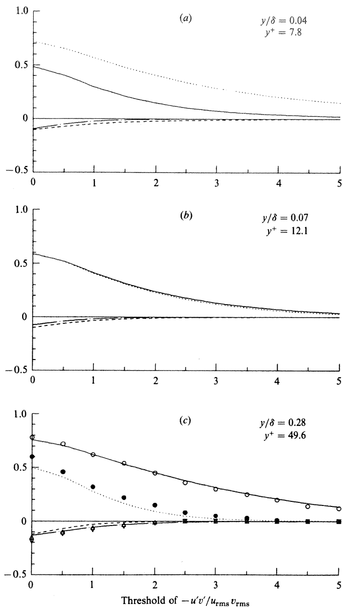
FIGURE 17. Fractional contribution to -\overline{u'v'} from each quadrant as a function of threshold; ----, first; —, second; — · —, third; ·····, fourth quadrants: (a) y^+ \approx 8 ; (b) 12; (c) 50. Symbols represent the interpolated data at y^+ = 50 from figure 3 of Alfredsson & Johansson (1984): \triangle , first; \circ , second; \nabla , third; \bullet , fourth quadrant.
