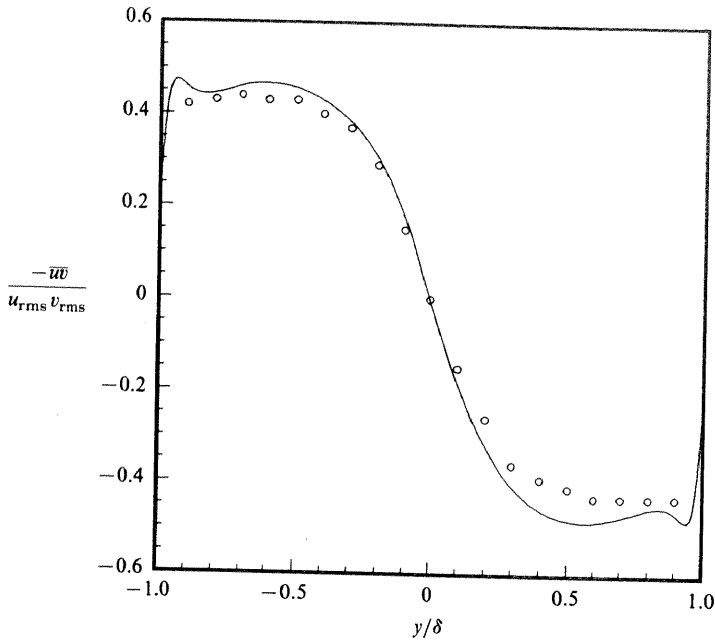
FIGURE 11. Correlation coefficient of u' and v' : —, computation; \circ , data from Sabot & Comte-Bellot (1976).
