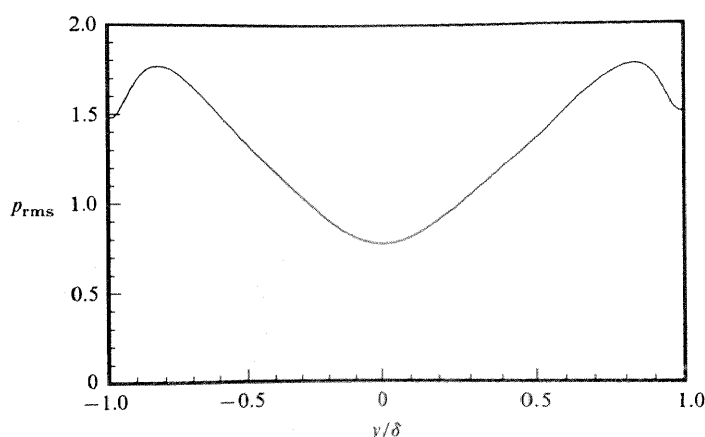
FIGURE 9. Root-mean-square pressure fluctuations normalized by the wall shear velocity, p_{\text{rms}}/\rho u_\tau^2 .
