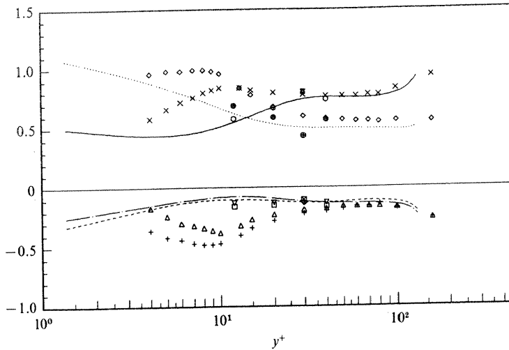
FIGURE 16. Reynolds shear stress from each quadrant normalized by the local mean Reynolds shear stress: ----, first; —, second; — · —, third; · · · ·, fourth quadrant. Symbols represent the experimental data: +, first; ×, second; Δ, third; ◇, fourth quadrant from Brodkey et al. (1974); □, first; ○, second; ▽, third; ●, fourth quadrant from Barlow & Johnston (1985); ⊠, first; ⊗, second; ⊕, third; ⊙, fourth quadrant from Willmarth & Lu (1972).
