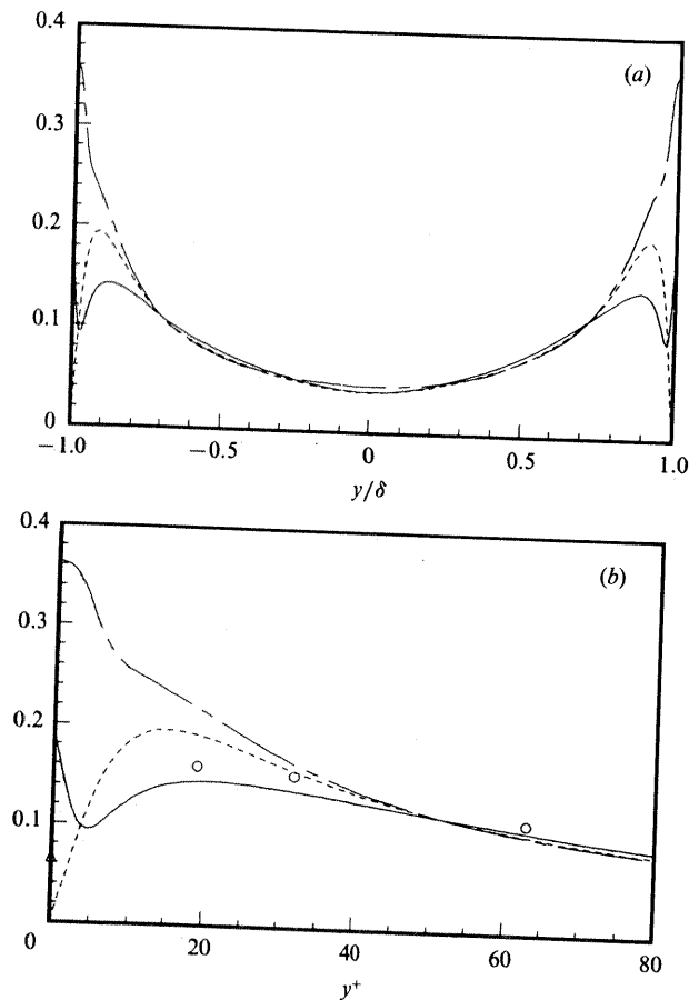
FIGURE 14. Root-mean-square vorticity fluctuations normalized by the mean shear. (a) In global coordinates: —, \omega_x v/u_\tau^2 ; ---, \omega_y v/u_\tau^2 ; - · -, \omega_z v/u_\tau^2 ; (b) in wall coordinates: \circ , \omega_x from Kastrinakis & Eckelmann (1983), \triangle , \omega_x at the wall from Kreplin & Eckelmann (1979).
