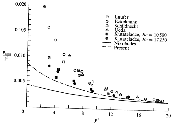
FIGURE 13. Comparison of the near-wall behaviour of the normal velocity fluctuation with experimental data from Finnicum & Hanratty (1985).
